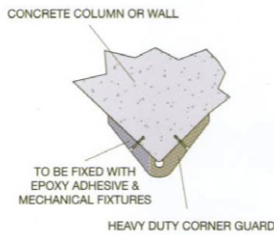
TYPE 'A' Without Clip and Yellow Strip
