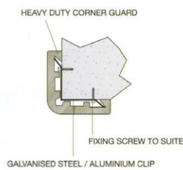
TYPE 'B' With Clip All Black
